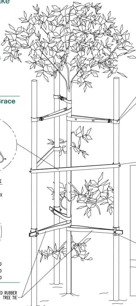
GREEN SLEEVES® THREE STAKE SYSTEM ISOMETRIC VIEW SCALE: NTS
