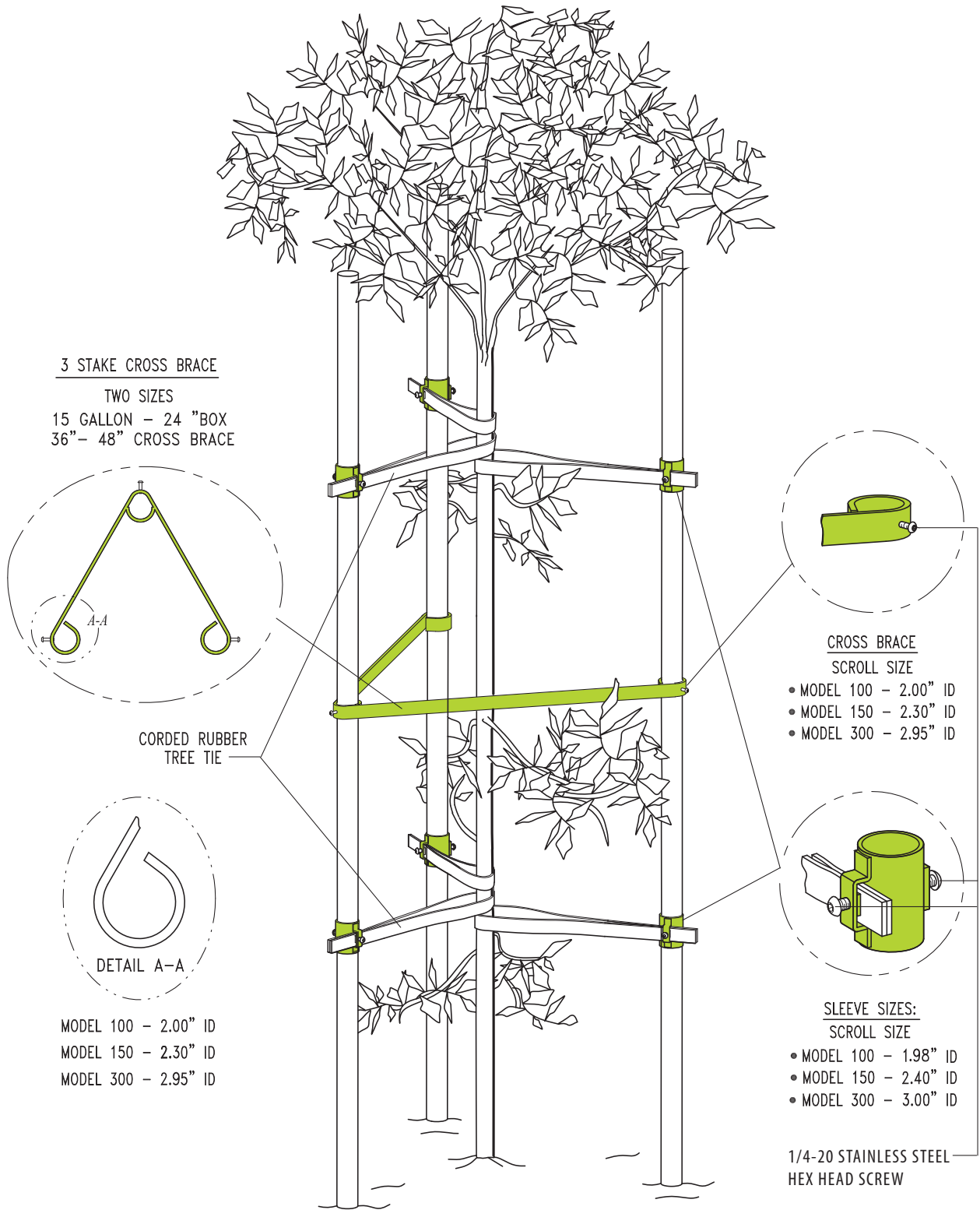
GREEN SLEEVES® THREE STAKE WITH ONE CROSS BRACE AND TWO TIES SYSTEM ISOMETRIC VIEW
